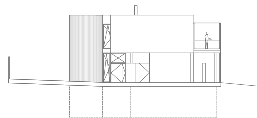
Alzado Norte/ North Elevation
