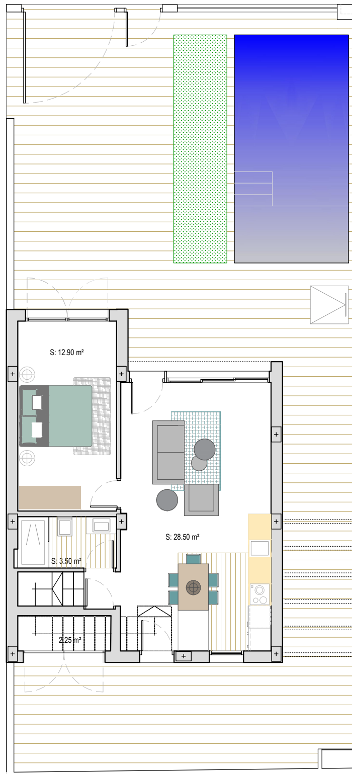
Ground floor
