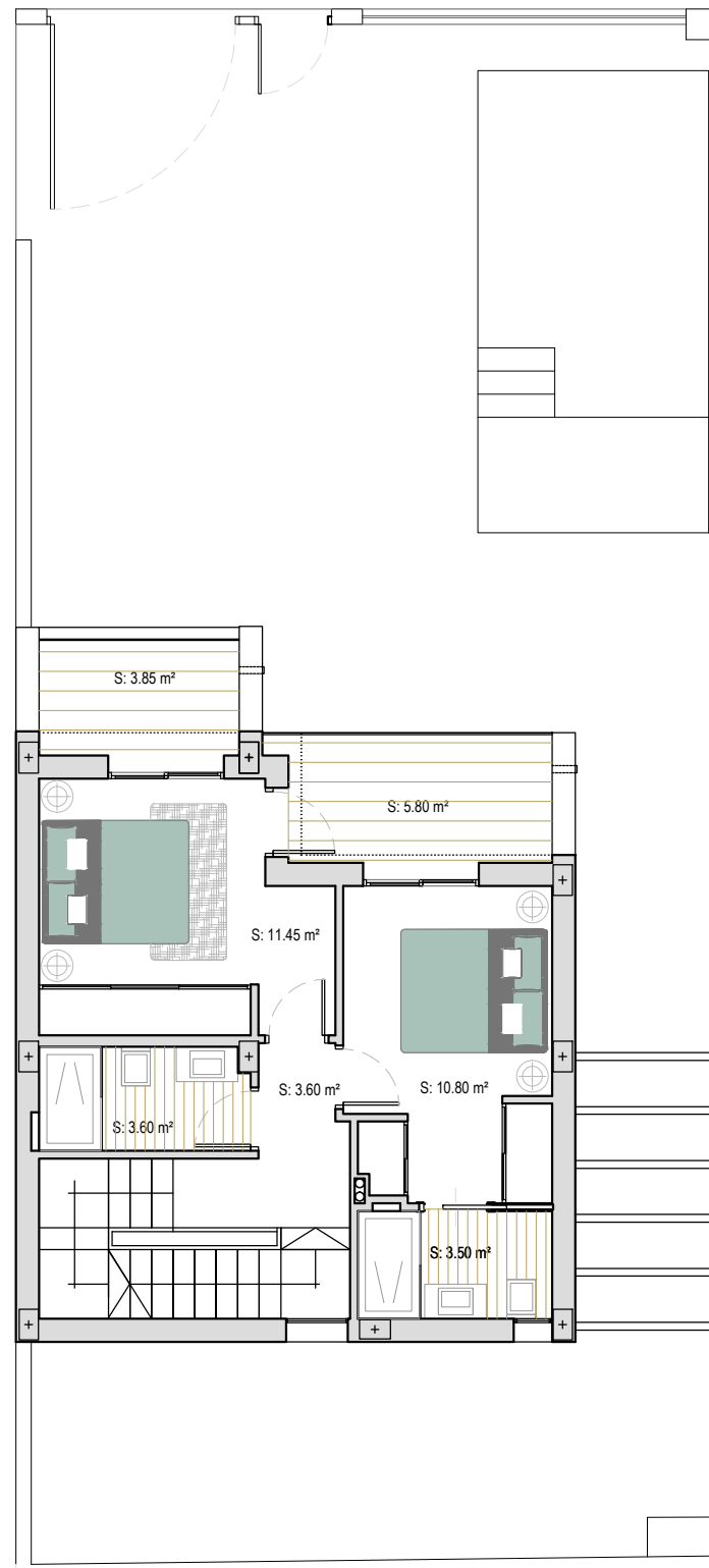
First floor
