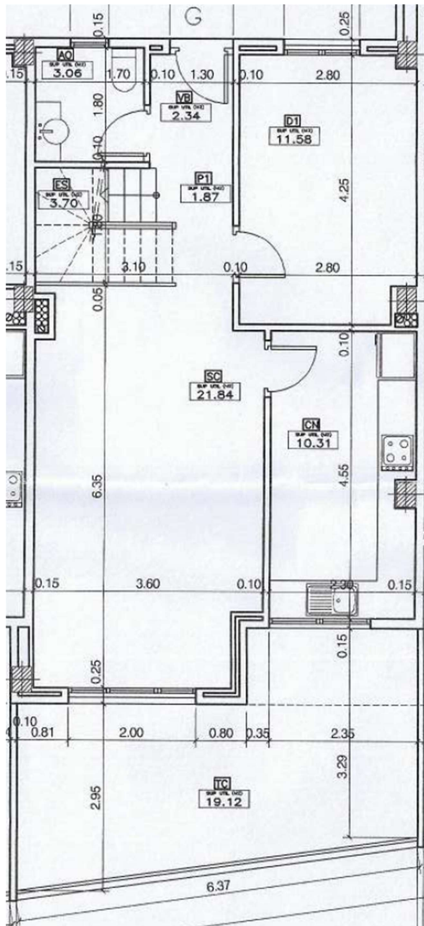
Dimensions and surfaces of the fourth floor
