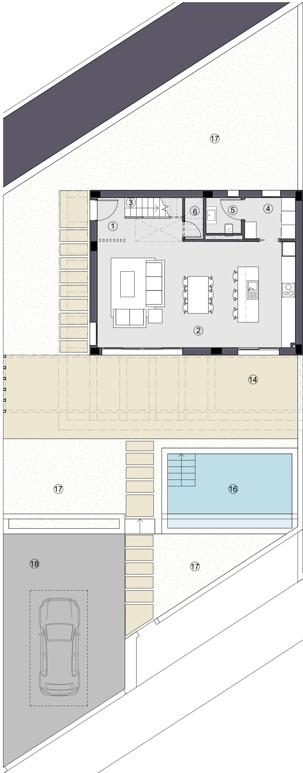
PLANTA BAJA / GROUND FLOOR
