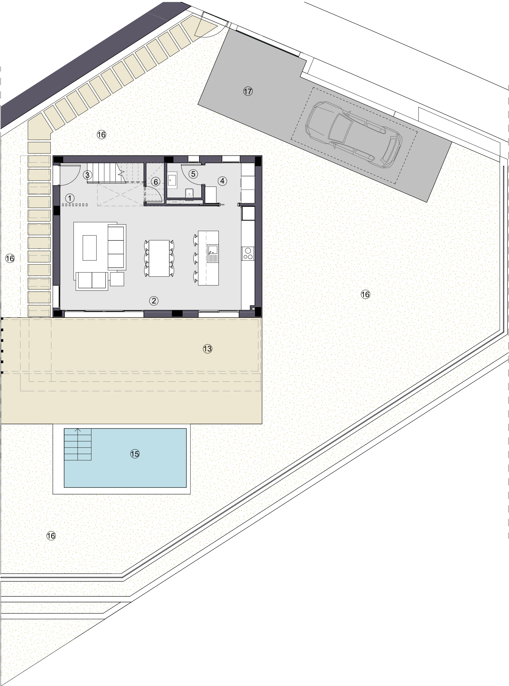
PLANTA BAJA / GROUND FLOOR
