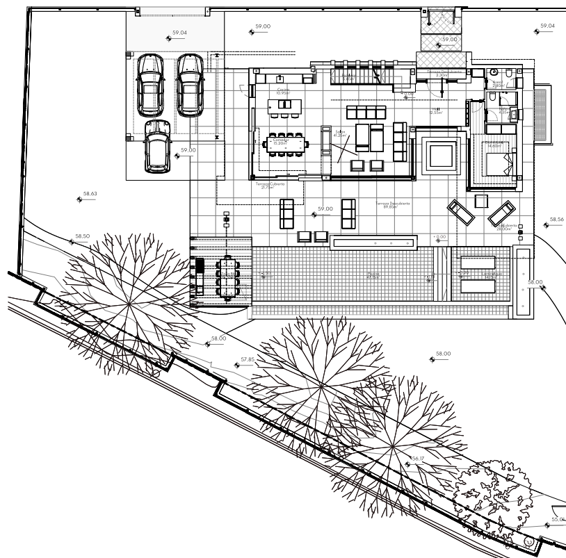
MAIN LEVEL
