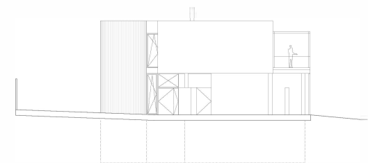
Alzado Norte/ North Elevation
