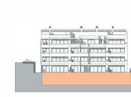
VISTA FRONTAL | FRONT VIEW
