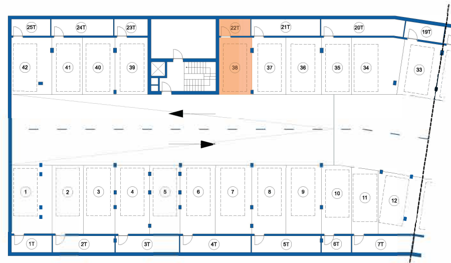
VISTA SUPERIOR | TOP VIEW
