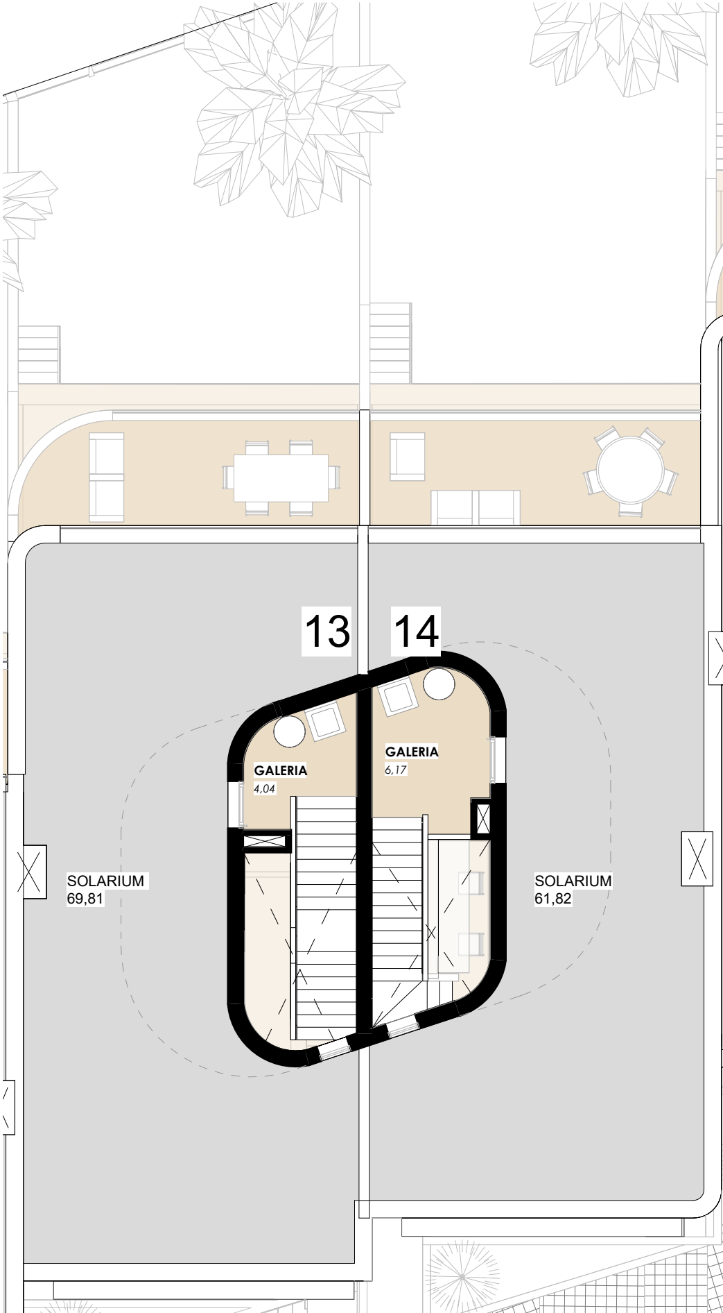
VIVIENDA 13-14_SOLARIUM/ APARTMENT 13-14_SOLARIUM 1 : 100
