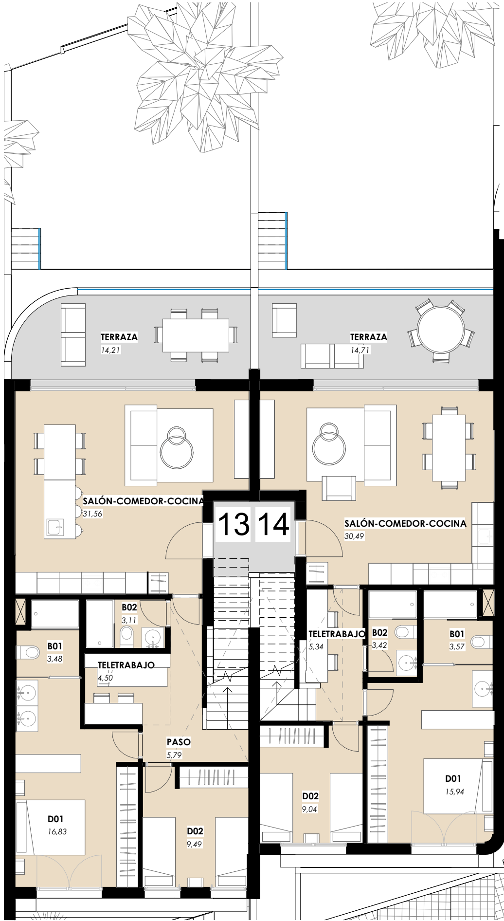
VIVIENDA 13-14_PLANTA PRIMERA/ APARTMENT 13-14_TOP FLOOR 1 : 100
