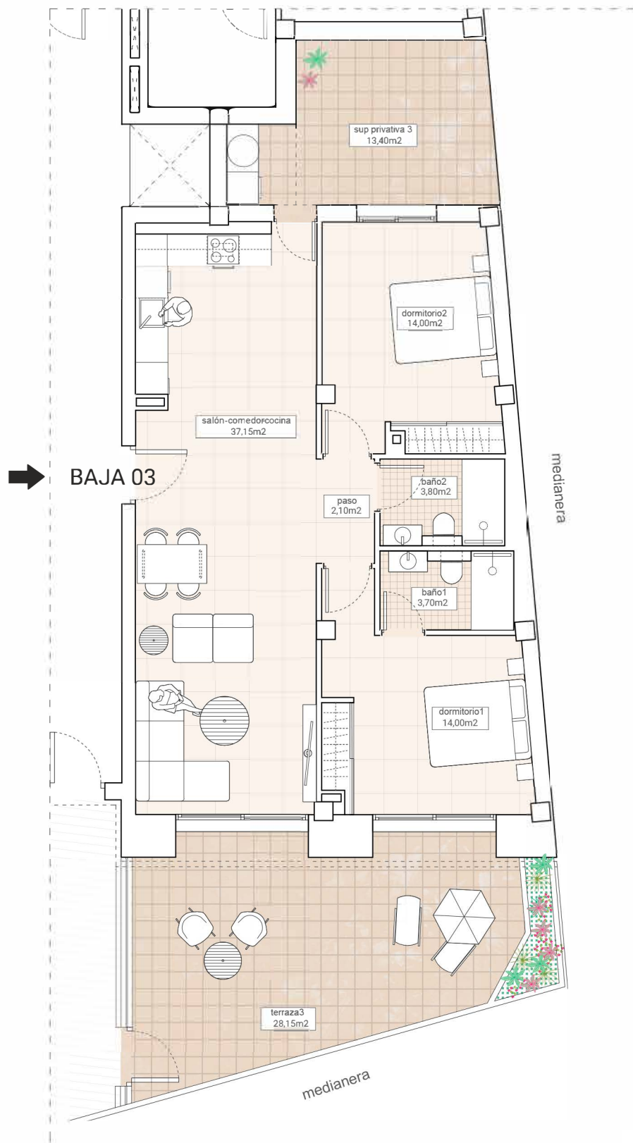
PLANTA BAJA/ GROUND FLOOR
