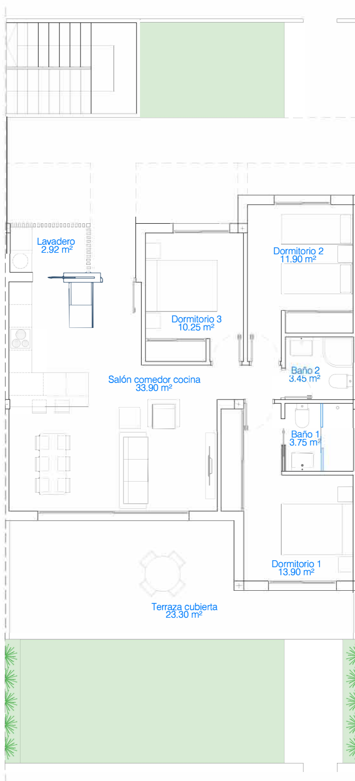
Ground Floor/ Planta Baja (E:1/100)
