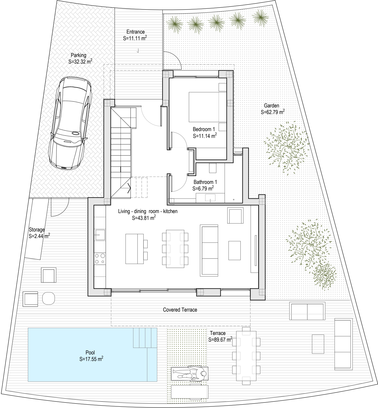
Ground floor
