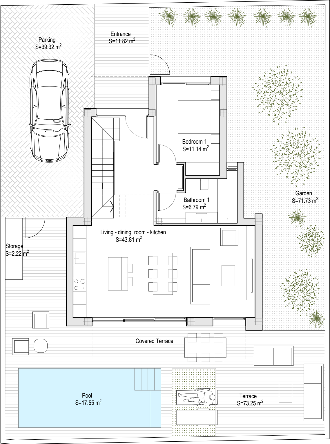
Ground floor
