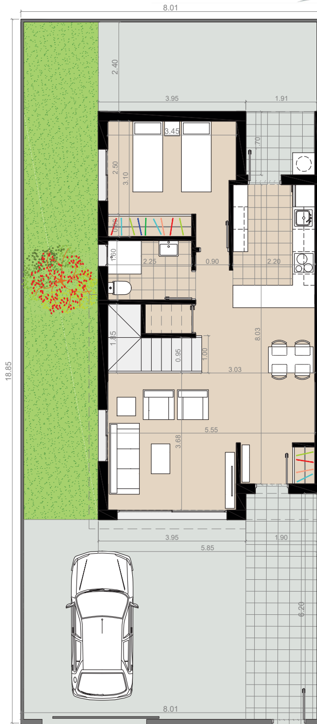
Planta baja / Ground floor
