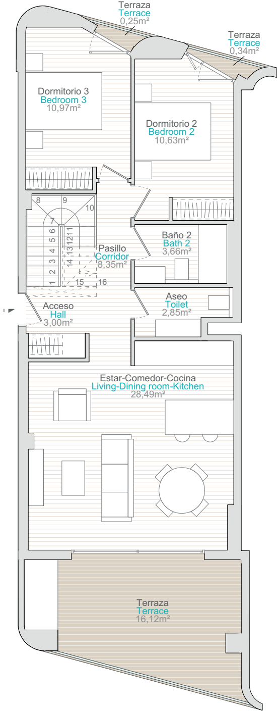
PLANTA 8 | Floor 8
