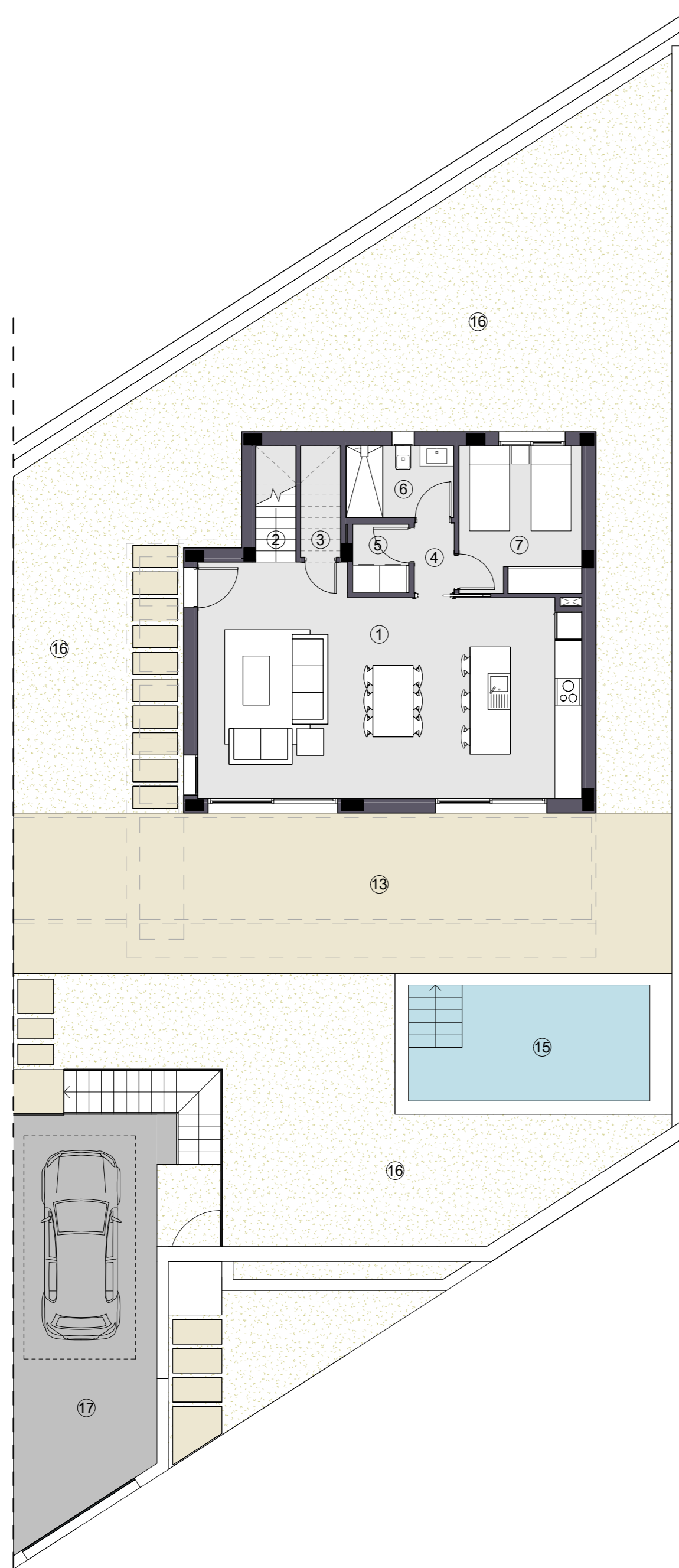
PLANTA BAJA / GROUND FLOOR
