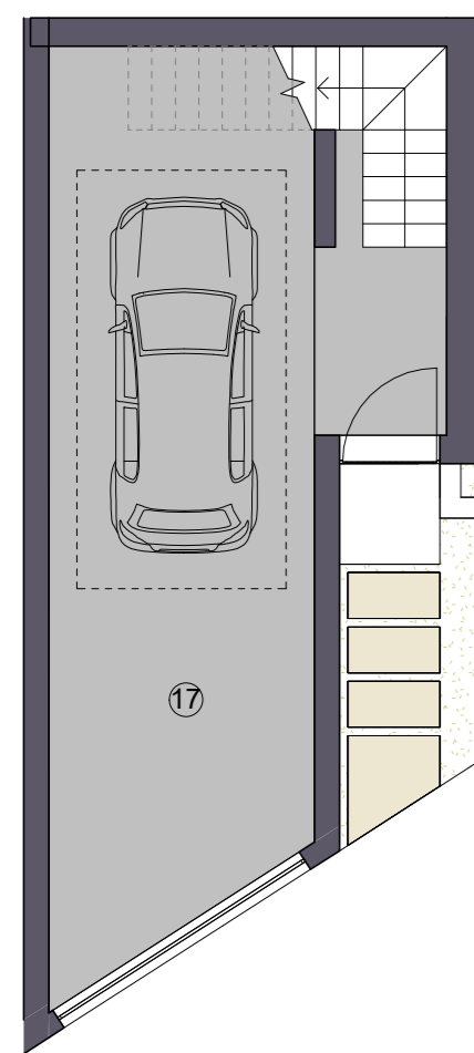
PLANTA SÓTANO / PARKING BASEMENT
