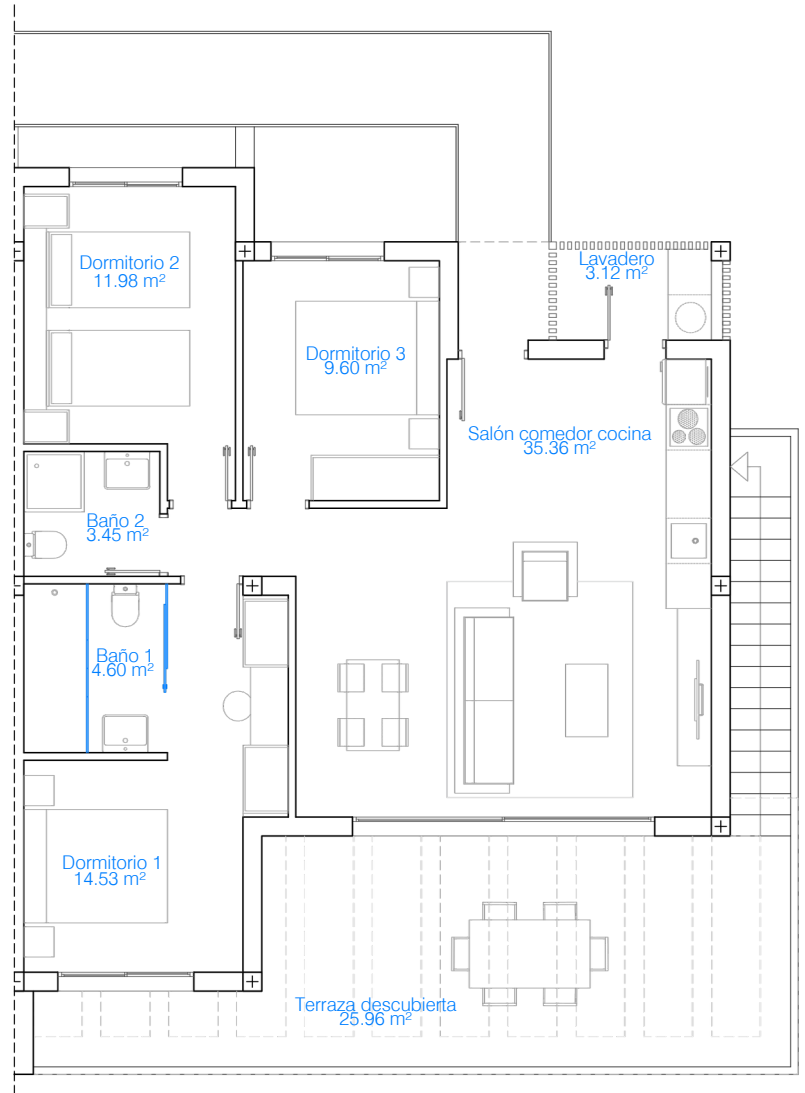
Top Floor/ Planta Alta (E:1/100)
