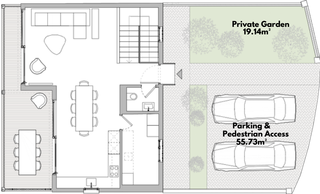
HOUSE + ENTRANCE + PARKING (Entrance Level)
