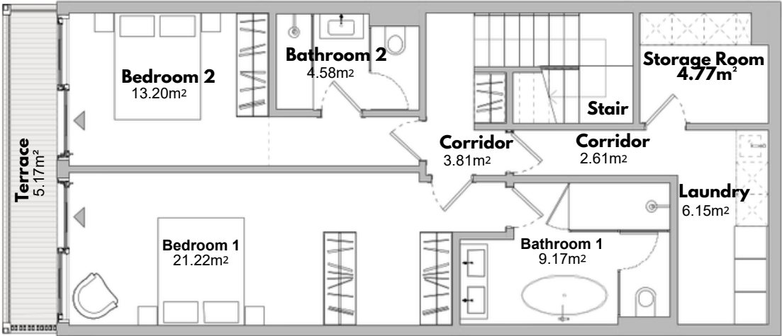
GROUND FLOOR PLAN (Lower Level)
