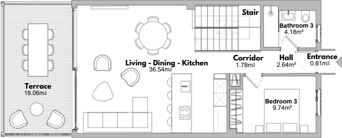
FIRST FLOOR PLAN (Entrance Level)
