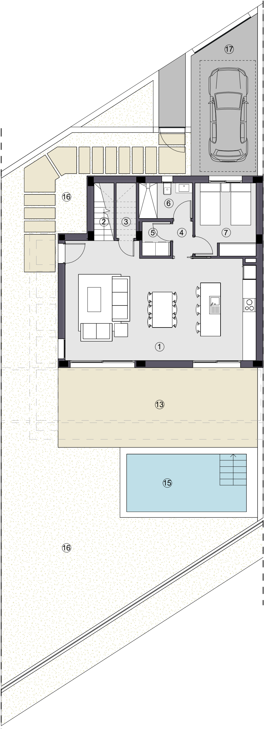
PLANTA BAJA / GROUND FLOOR
