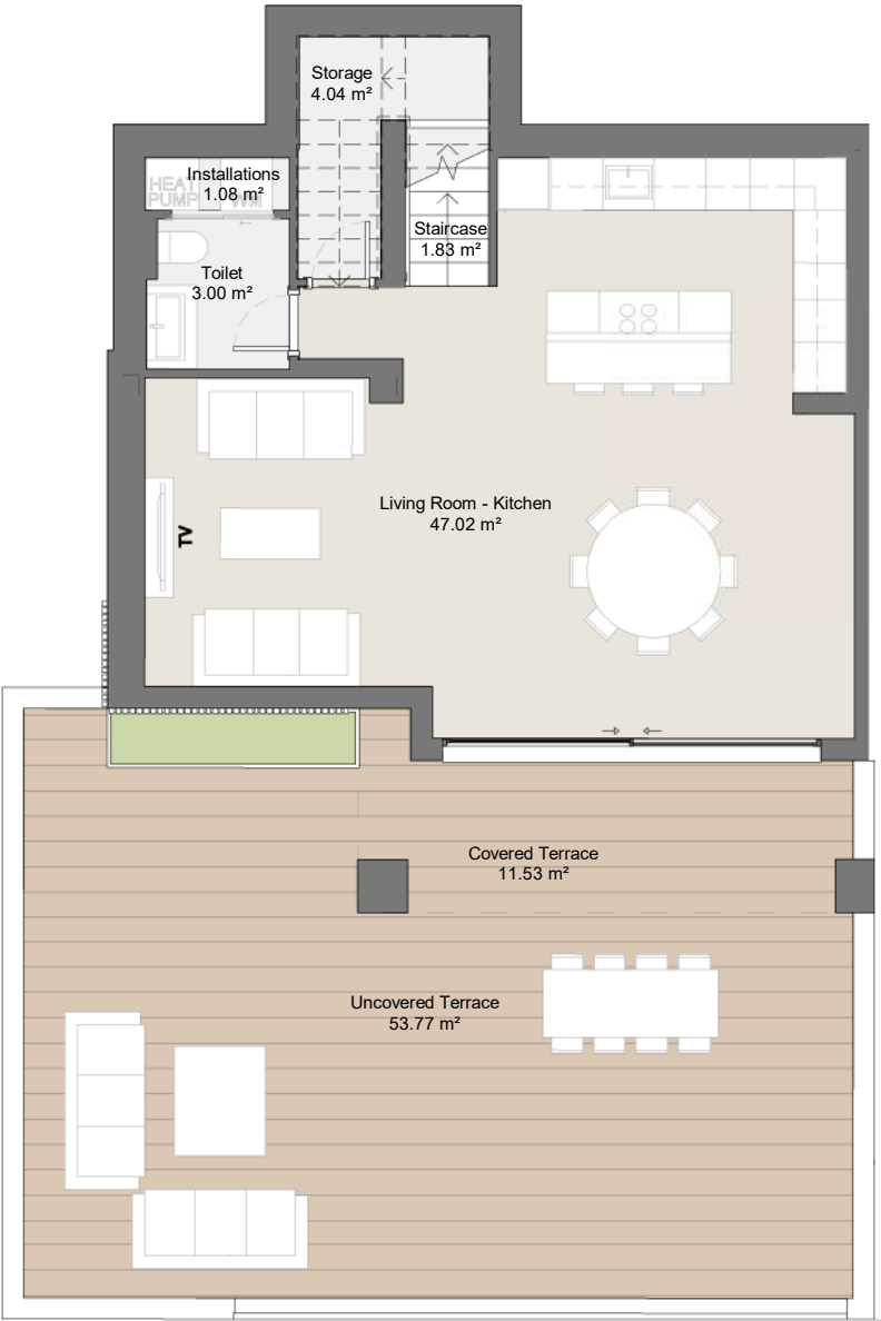
GROUND FLOOR
