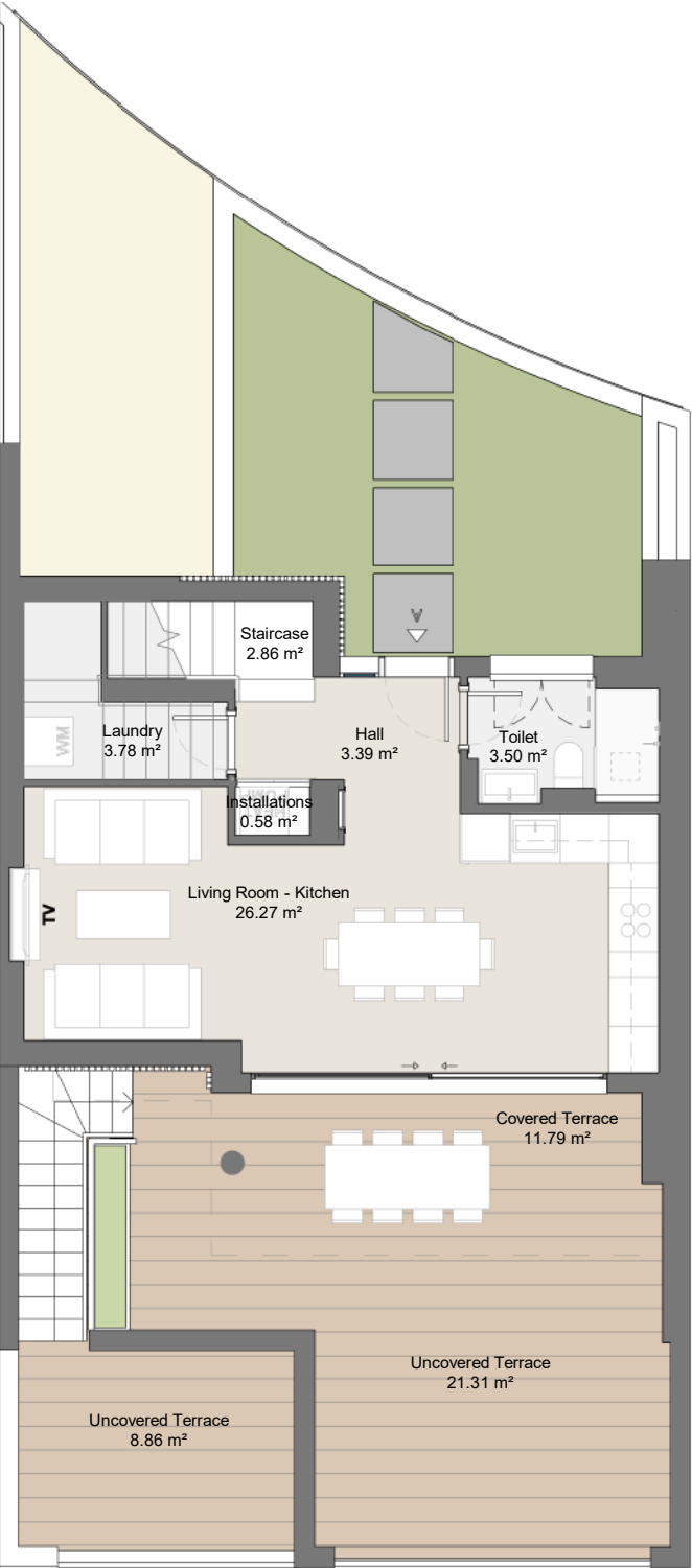
GROUND FLOOR
