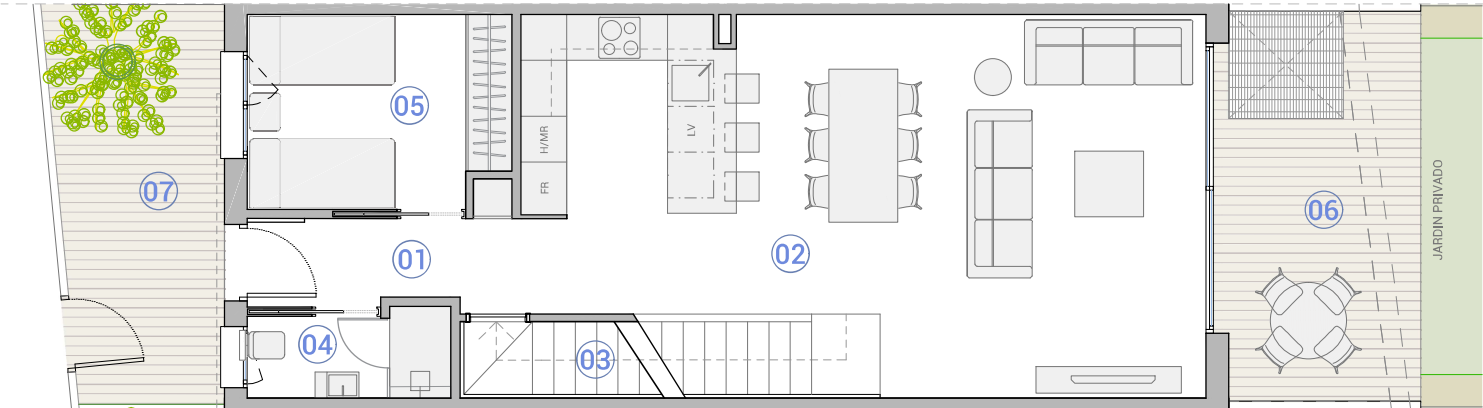
Planta / Floor Baja / Ground
