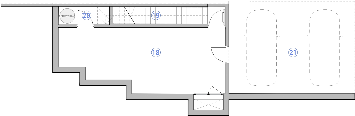
Planta / Floor Baja / Ground
