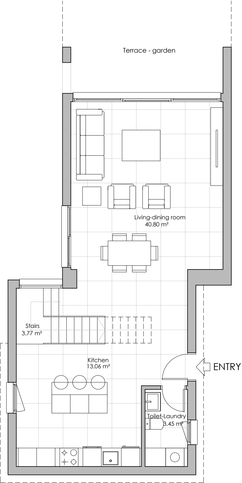
GROUND FLOOR
